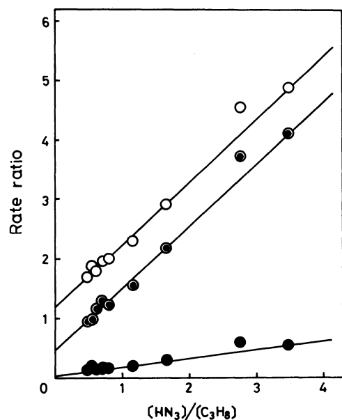
Fig. 9. Plots of the rate ratios vs. [\text{HN}_3]/[\text{C}_3\text{H}_8] . O, [(\phi_{\text{H}_2} + \phi_{\text{N}})/4] / [\phi_{\text{CH}_4} - k_{10}/(k_5 + k_6)] / \alpha ; ◐, [(\phi_{\text{N}_2} + \phi_{\text{H}_2}) / (\phi_{\text{CH}_4} - (3k_5 + 3k_8 + k_{10})/(k_5 + k_6))] / 4\alpha ; ●, [\phi_{\text{H}_2} / (\phi_{\text{CH}_4} - k_{10}/(k_5 + k_6))] / \alpha - \beta .
